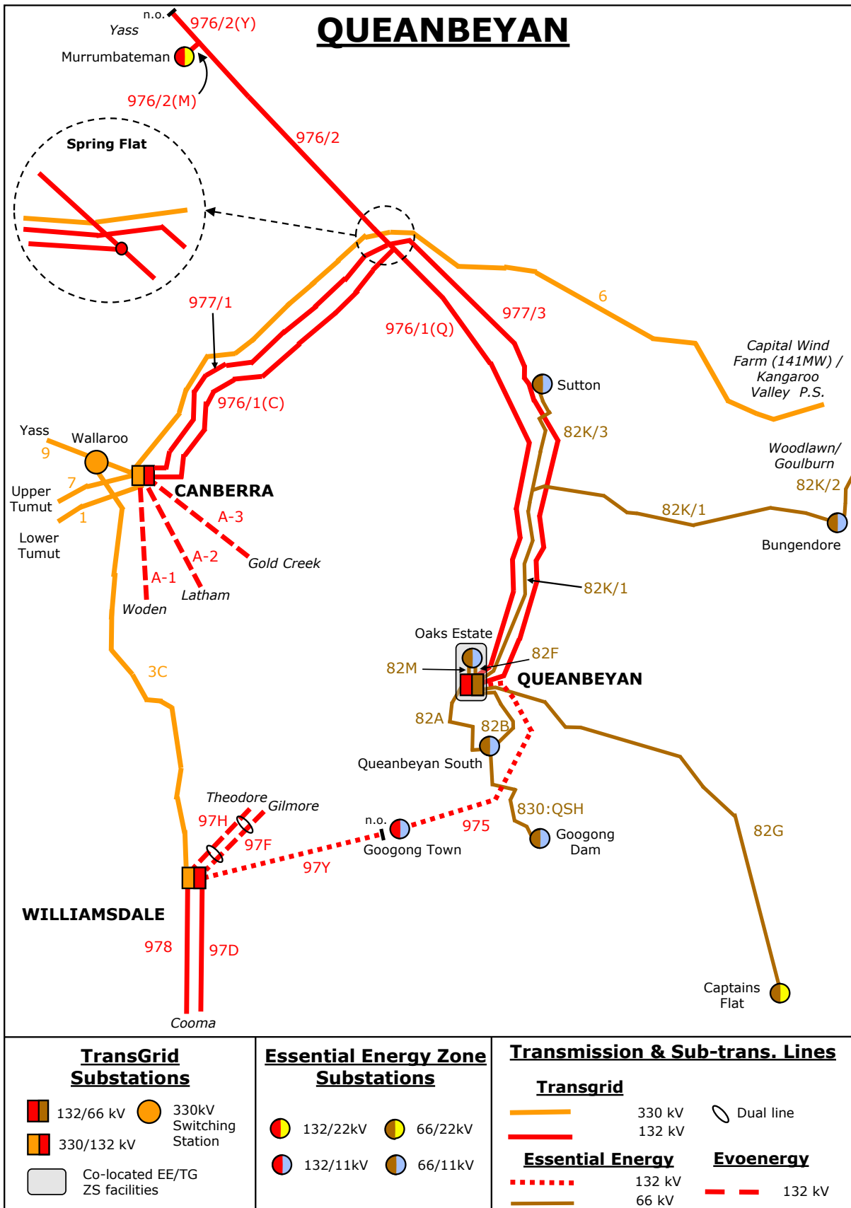
Sub-transmission Single Line Diagram of Queanbeyan area
