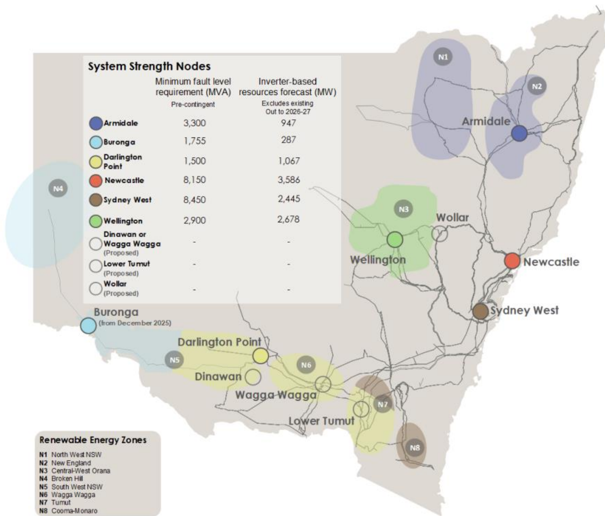
Figure 5 - System strength node location and system strength standard in New South Wales
