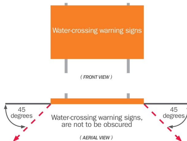
Figure 9. Clearance dimensions for water crossings
