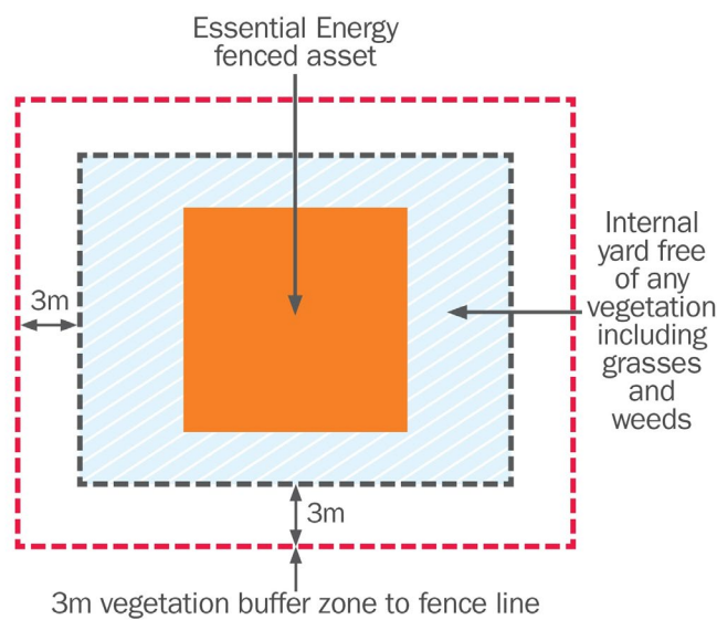
Figure 6. Clearance dimensions for fenced assets (includes SAPS)
