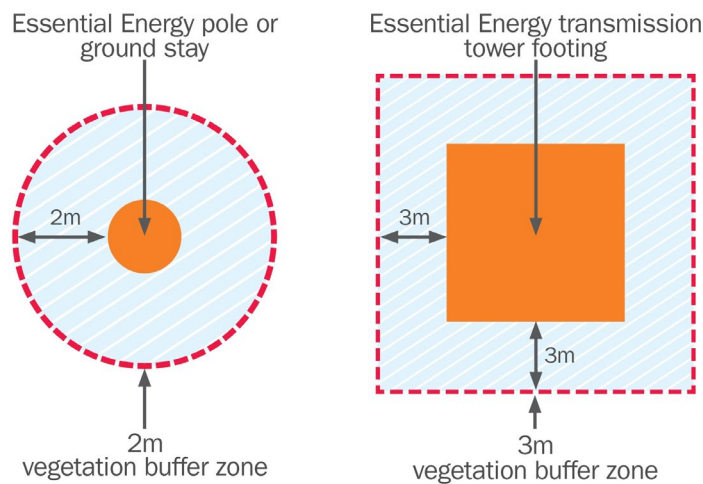
Figure 8. Clearance dimensions for stays poles and towers
