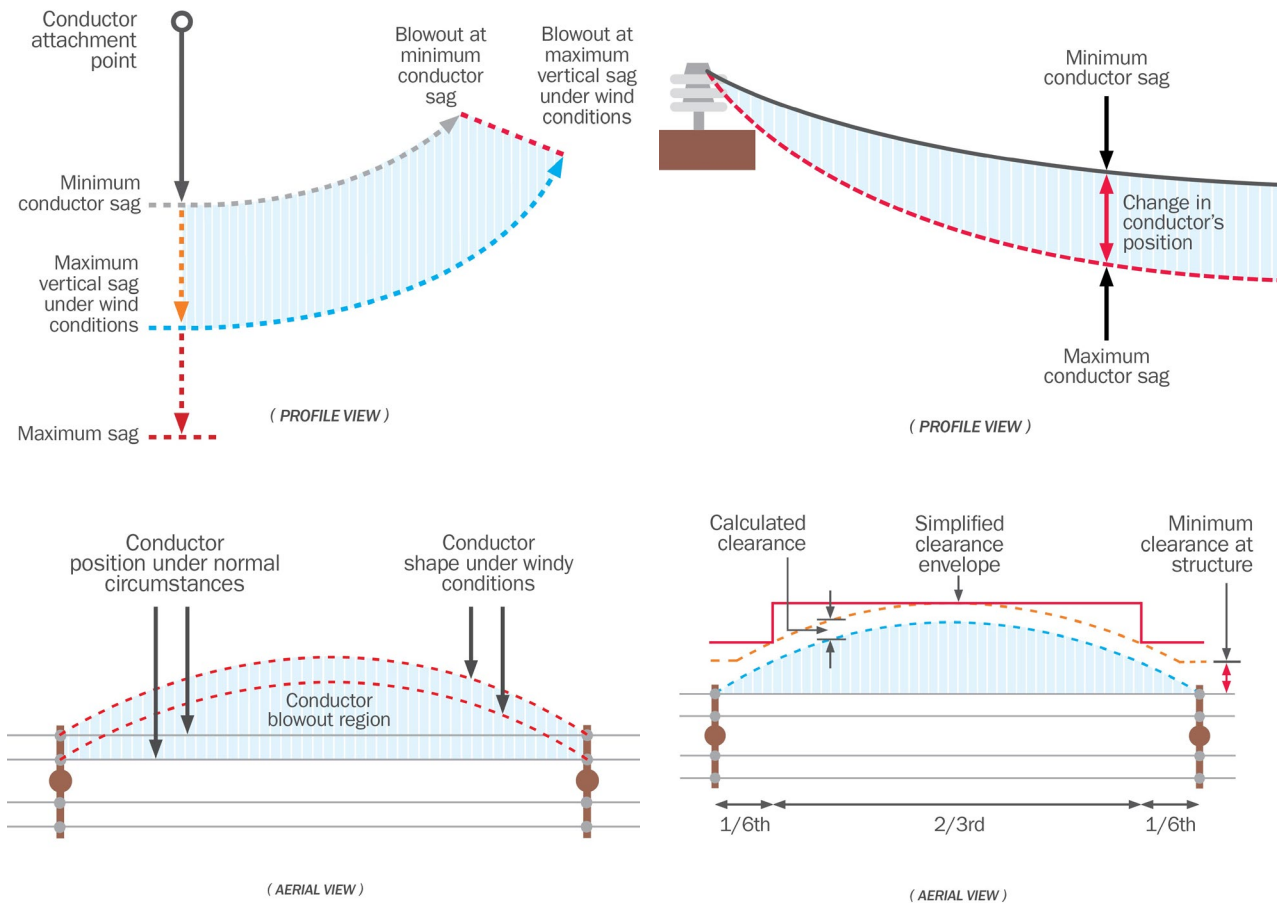
Figure 3. Conductor movement and simplified clearance envelope
